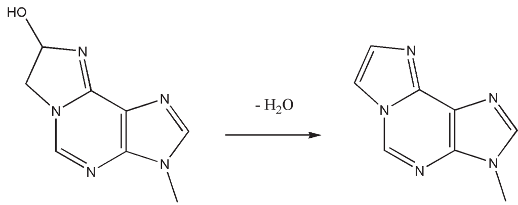
1,N 6 -α-hydroxyethanoadenine
