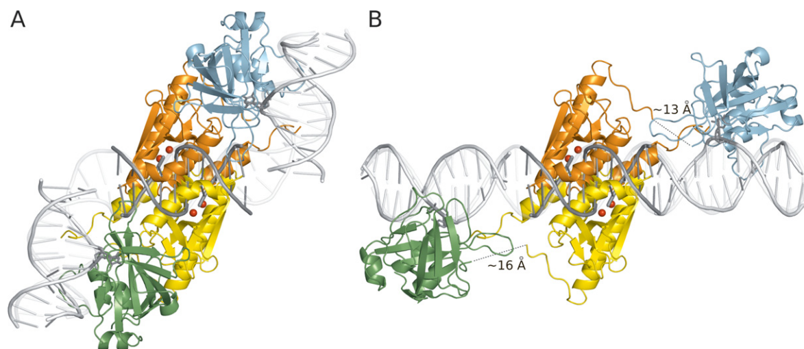
Figure 5. Models for the PvuRtsII dimer bound to target DNA. (A) Bent DNA and PvuRtsII with linker conformation observed in the crystal. (B) Straight DNA and PvuRtsII with adjusted interdomain linker. Nuclease domains (with modeled metal ions) were placed on the DNA based on the superposition with the NgoMIV-DNA complex (37). The binding mode of the DNA to the SRA domain is modeled after the UHRF1-DNA complex.
