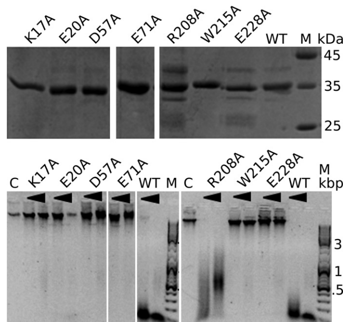
Figure 3. Effect of mutations on PvuRtsII activity. PvuRtsII and its variants were either analyzed for protein purity by SDS-PAGE and Coomassie staining (top, 3 \mu g per lane) or used to digest 240 ng of phage T4 DNA, which was then analyzed by gel electrophoresis in a 1% agarose gel and stained with Gel Red. For each variant, two protein amounts (0.1 \mu g, left; 1 \mu g, right) were tested.
